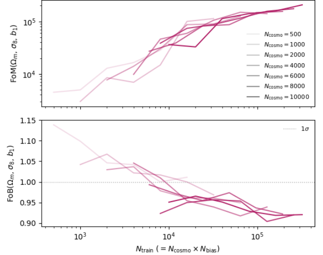
Figure 9. Convergence of the inference with training set size, for P_{gg}(k) + B_{ggg}(k_1, k_2, k_3) + P_{gm}(k) on the coverage test set for the three key parameters \Omega_m , \sigma_8 , and b_1 combined. The top panel shows the figure of merit (FoM), and the bottom panel shows the figure of bias (FoB), normalized by the 68th percentile of the \chi^2 distribution for three dimensions (corresponding to the three parameters); the median values over the coverage set are shown. The opacity indicates the number of training cosmologies. Increasing the number of training points increases the precision significantly until N_{\text{train}} \sim 20,000 and then more marginally, with the number of cosmologies and bias parameter sets contributing similar precision; the bias also plateaus around N_{\text{train}} \sim 20,000 , with the number of cosmologies mattering more than the number of bias parameters for smaller N_{\text{train}} . ksf: make higher res
