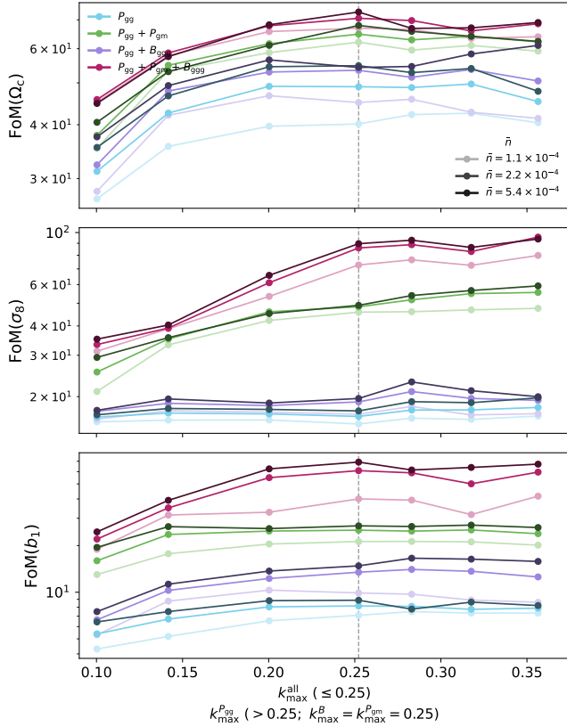
Figure 9. Scale dependence of the figure of merit (FoM) for the three key parameters for the SHAME out-of-distribution mock, with varying number density. The k_{\max} is for all three statistics for k < 0.25 ; for k > 0.25 , we fix k_{\max}^{\text{Pgm}} = k_{\max}^{\text{Bgg}} = 0.25 and only include higher k for P_{gg}(k) . Precision increases with scale, particularly for \sigma_8 for P_{gg}(k) + P_{gm}(k) + B_{ggg}(k_1, k_2, k_3) . ksf: make legends, axis labels bigger
