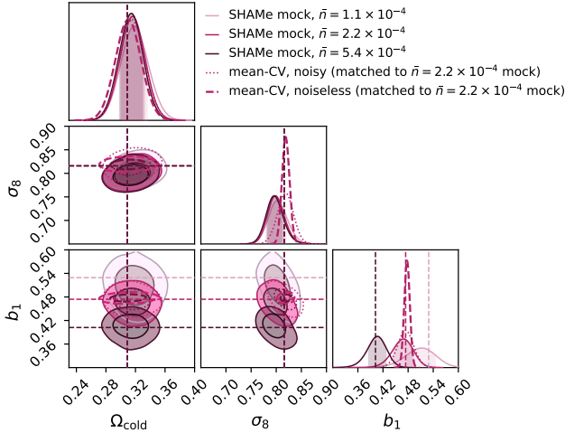
Figure 7. Posteriors for P_{gg}(k) + B_{ggg}(k_1, k_2, k_3) + P_{gm}(k) for the key parameters, for varying number density and noise models. The filled contours show the results for the SHAMe OOD mock data with different number densities. The dotted contours show inference on the mean of the cosmic variance test set, which was matched to the fiducial \bar{n} = 2.2 \times 10^{-4} (h^{-1}\text{Mpc})^{-3} SHAMe mock; the dashed contour shows that same set but generated without any noise, and inferred assuming noiseless data.
