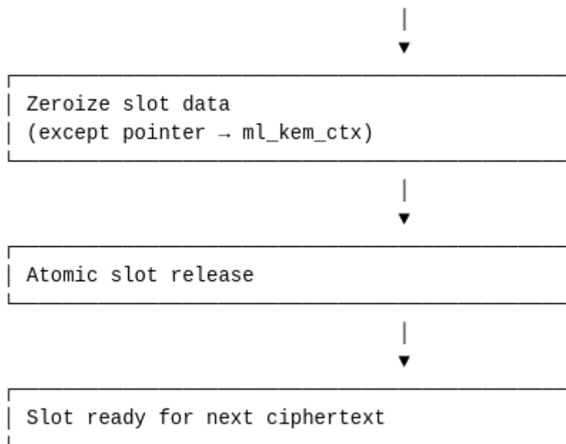
4.15.b. Runtime Decapsulation Flow(continue)
