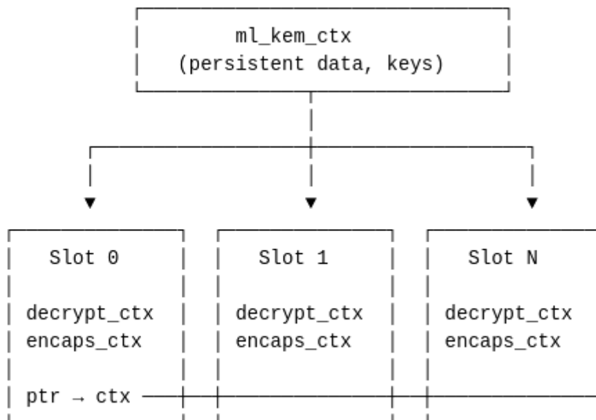
4.16. Memory Model
