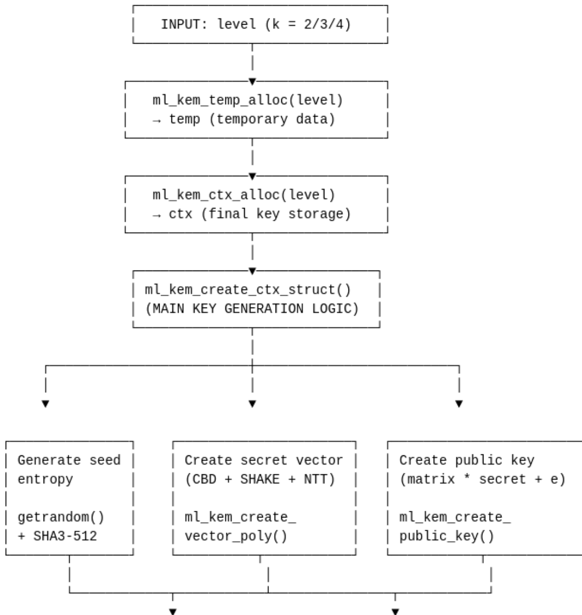
4.3a — General key generation scheme
