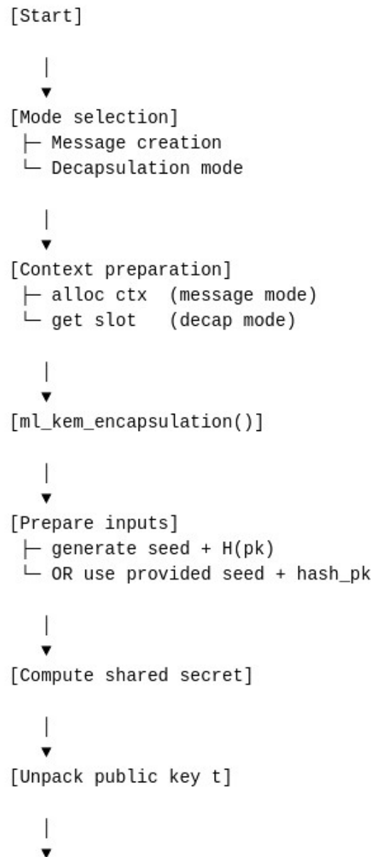
4.5a. Encapsulation execution sequence
