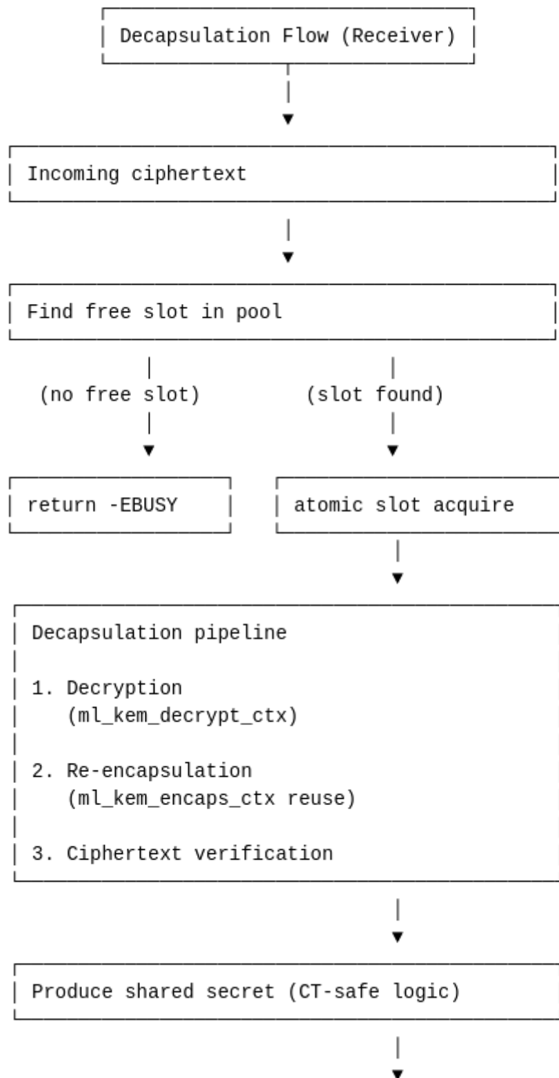
4.15.a. Runtime Decapsulation Flow
