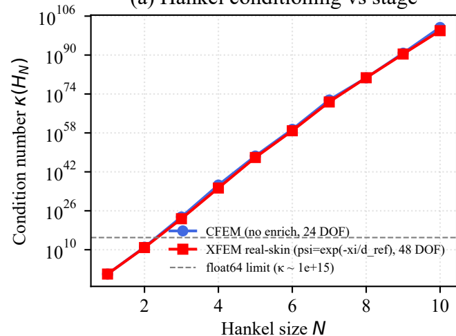
(a) Hankel conditioning vs stage
