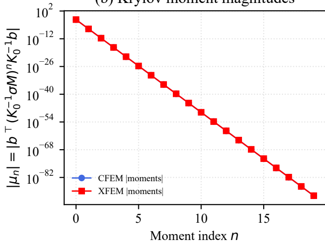
(b) Krylov moment magnitudes
