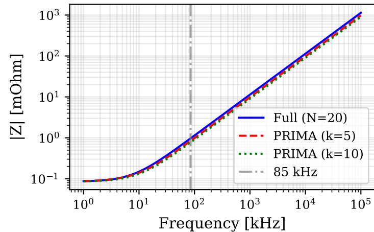
(a) Impedance magnitude
