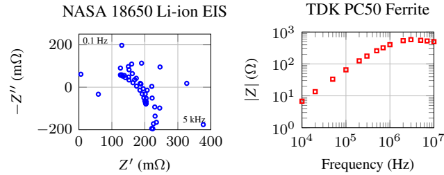
Real-world EIS data used for URN validation. Left: NASA 18650 Li-ion battery showing semicircle (charge transfer) and Warburg tail (diffusion). Right: TDK PC50 MnZn ferrite showing frequency-dependent impedance with Cole-Cole relaxation peak near 3 MHz.
