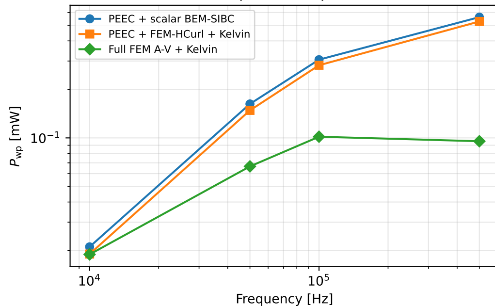
Workpiece dissipation
