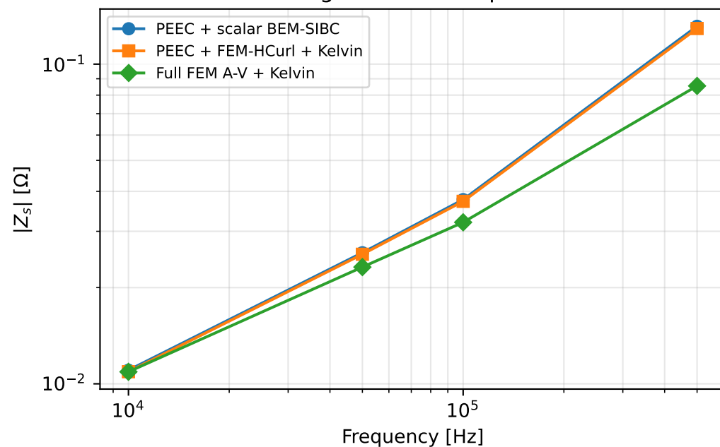
Converged surface impedance
