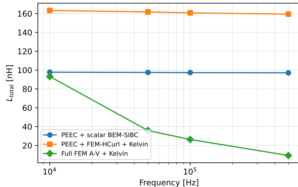
Total inductance
