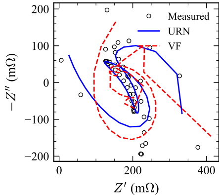
(a) Nyquist plot
