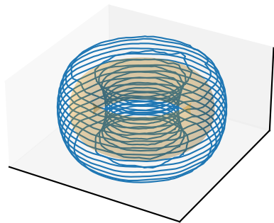
(a) current-potential coil + plasma
