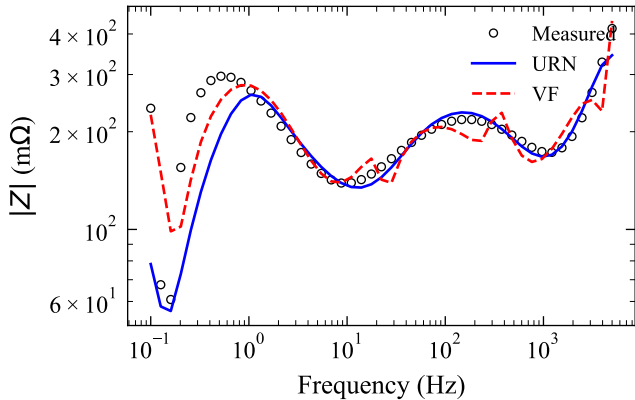
(b) Bode magnitude
