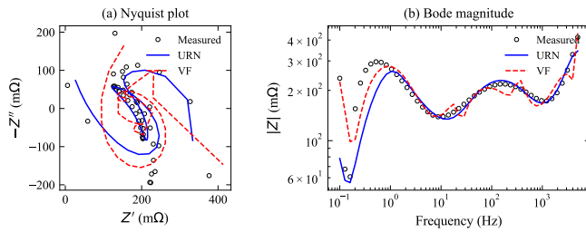
NASA 18650 Li-ion battery EIS validation. (a) Nyquist plot showing semicircle (charge transfer) and Warburg tail (diffusion). (b) Bode magnitude plot. Open circles: measured data; solid blue: URN fit; dashed red: Vector Fitting. URN achieves 9.1% lower NRMSE than VF.
