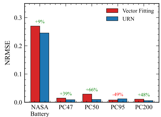
FIGURE 3. URN vs Vector Fitting NRMSE comparison across five real-world datasets. URN outperforms VF on 4/5 datasets (average 22.8% improvement). PC95 ferrite favors VF due to near-ideal Debye behavior.
