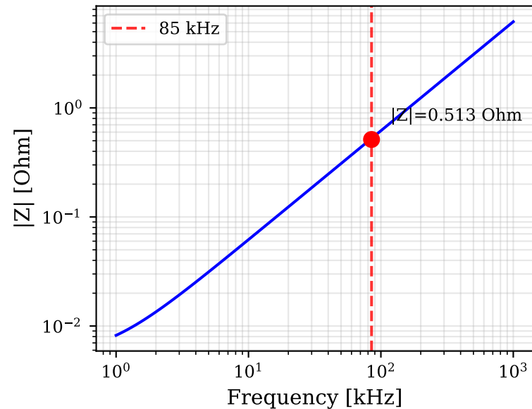
(a) Impedance magnitude
