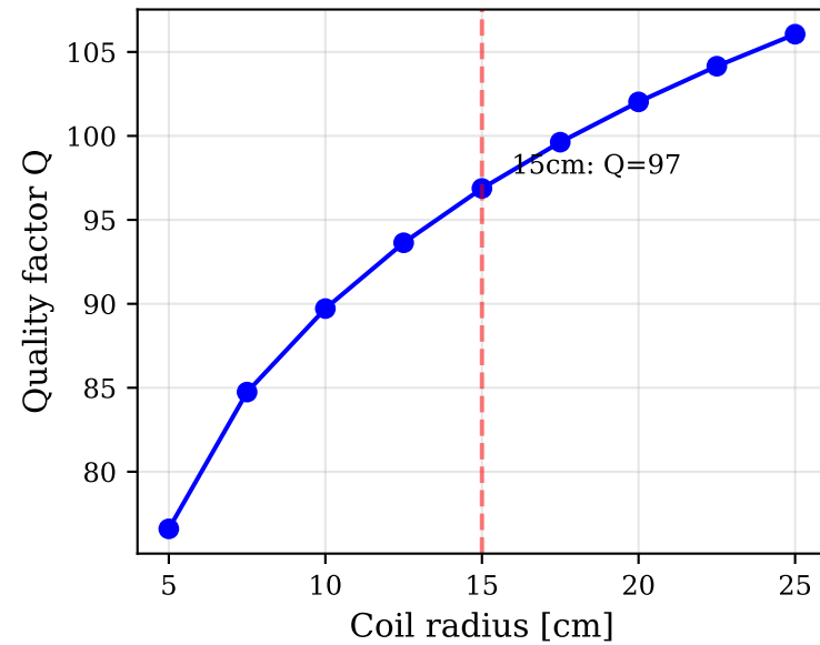
(c) Q factor at 85 kHz
