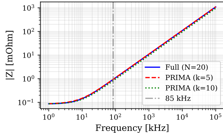
(a) Impedance magnitude
