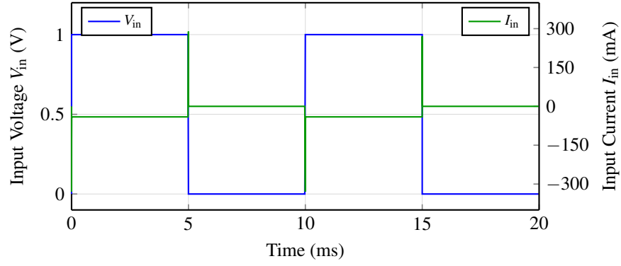
Figure 1: Transient response of URN equivalent circuit: input voltage pulse and resulting current. Data source: Actual LTspice simulation (not analytical approximation).
