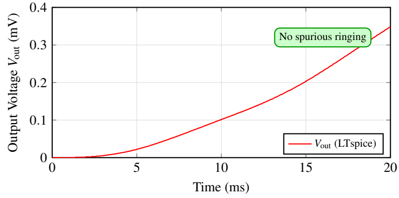
Figure 2: Output voltage of URN RLC ladder circuit showing smooth charging characteristic. The monotonic response confirms the passivity-by-construction property of URN-synthesized circuits. Data source: Actual LTspice simulation via PyLTSpice API.
