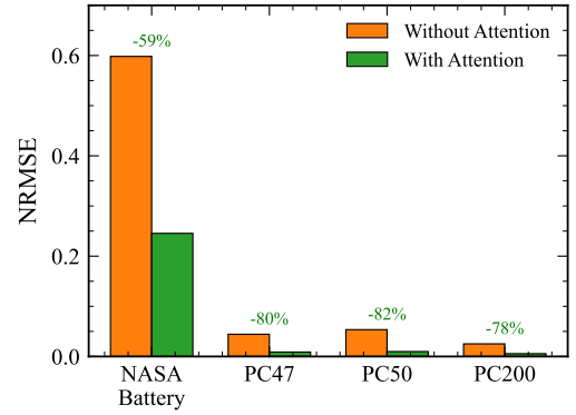
FIGURE 4. Ablation study: NRMSE comparison with and without frequency-dependent attention mechanism. Attention provides 59–82% accuracy improvement by automatically emphasizing relevant basis functions at different frequency ranges.
