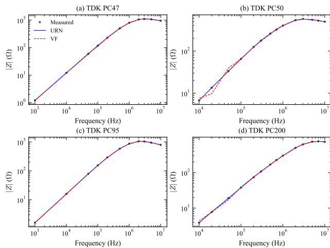
FIGURE 2. TDK MnZn ferrite impedance validation on four materials: (a) PC47, (b) PC50, (c) PC95, (d) PC200. Open circles: datasheet values; solid blue: URN fit; dashed red: Vector Fitting. URN outperforms VF on PC47/PC50/PC200 (Cole-Cole relaxation), while VF is superior on PC95 (near-ideal Debye behavior).
