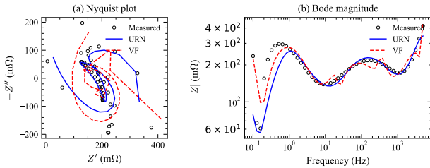
FIGURE 1. NASA 18650 Li-ion battery EIS validation. (a) Nyquist plot showing semicircle (charge transfer) and Warburg tail (diffusion). (b) Bode magnitude plot. Open circles: measured data; solid blue: URN fit; dashed red: Vector Fitting. URN achieves 9.1% lower NRMSE than VF.
