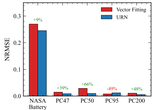
FIGURE 3. URN vs Vector Fitting NRMSE comparison across five real-world datasets. URN outperforms VF on 4/5 datasets (average 22.8% improvement). PC95 ferrite favors VF due to near-ideal Debye behavior.
