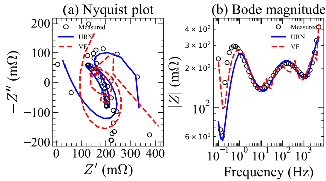
FIGURE 1. NASA 18650 Li-ion battery EIS validation. (a) Nyquist plot showing semicircle (charge transfer) and Warburg tail (diffusion). (b) Bode magnitude plot. Open circles: measured data; solid blue: URN fit; dashed red: Vector Fitting. URN achieves 9.1% lower NRMSE than VF.
