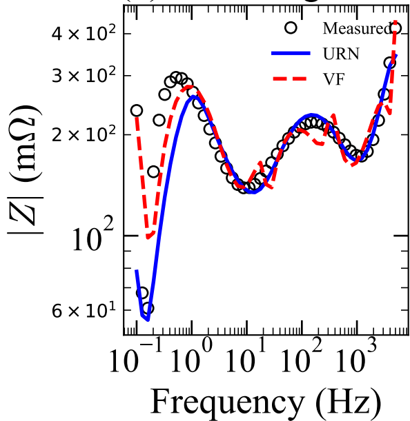
(b) Bode magnitude
