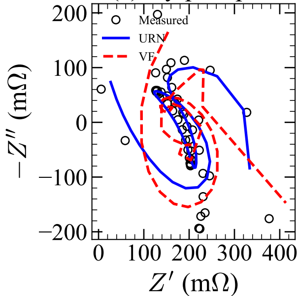
(a) Nyquist plot
