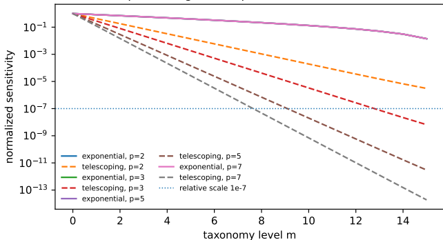
Depth-wise gradient profiles ( D=16 , s=0.85 )
