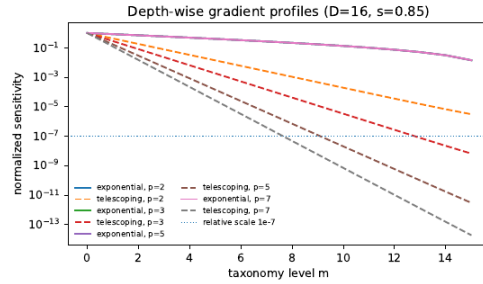
Figure 1: Finite-depth gradient profiles. The telescoping extension carries additional geometric attenuation across depth.
