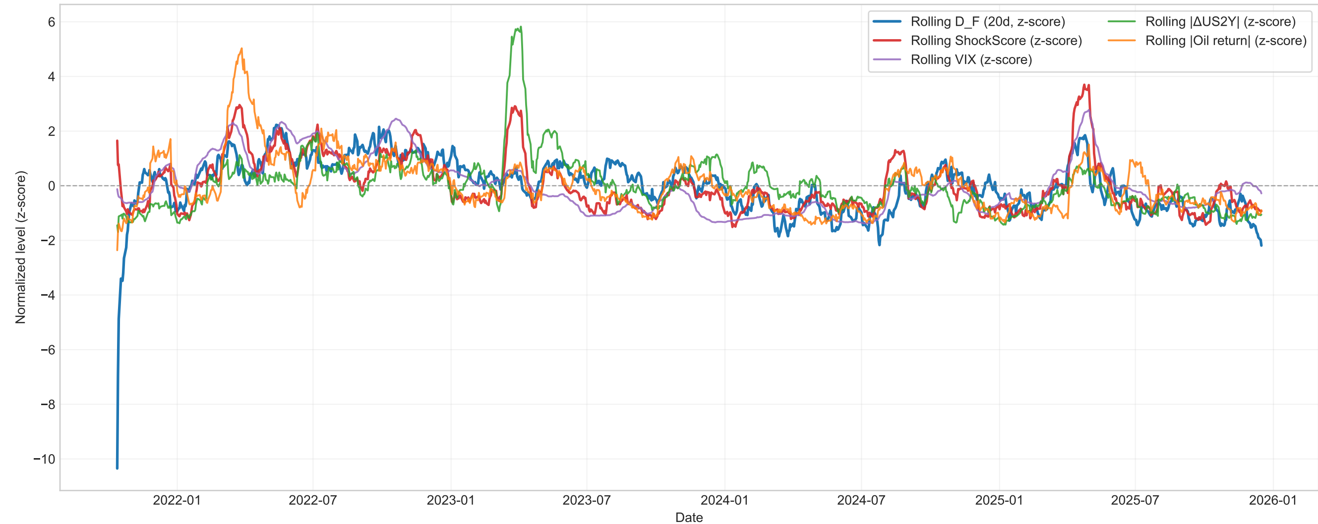
Macro Volatility vs Dynamic Graph Reconfiguration
