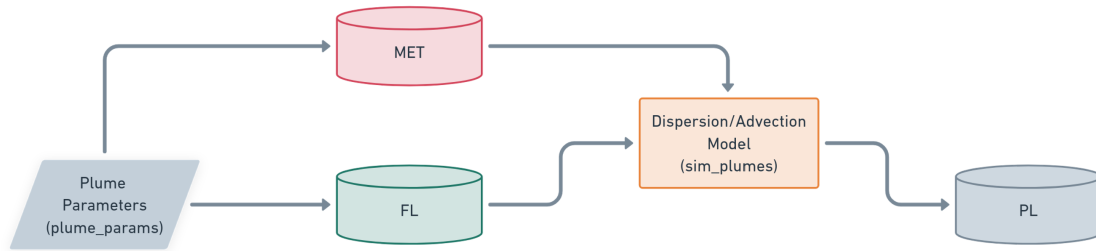
Figure 5.9: Process flow diagram for the Dispersion/Advection Model. MET is updated by passing plume_params to it, assigning additional dispersion properties to the dataset. The 2 nd gen. MET and FL datasets are passed to the sim_plumes model which simulates the advection and dispersion of plume waypoints. Plume position and Gaussian dispersion data is then attached to the Plume Dataset.
