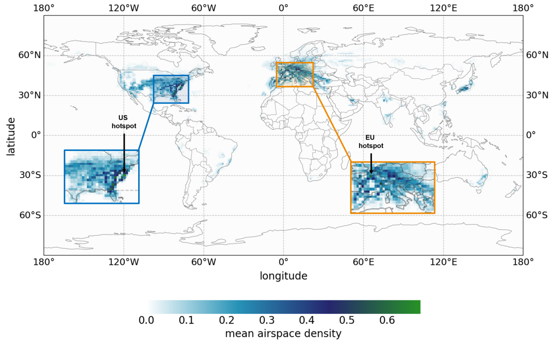
Figure 3.3: Global heatmap of mean air traffic density. Snapshots of air traffic data were taken at the first second of every hour throughout 01/2022. Mean values are significantly lower than peak values due to large variations in aviation demand throughout the course of each day.
