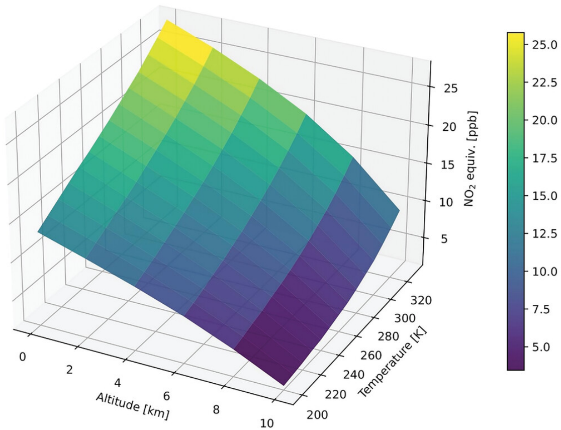
Figure 4.1: Calculated [ \text{NO}_2 ] equiv using simple kinetic equation (Equation (4.2)) at different temperatures and altitudes.
