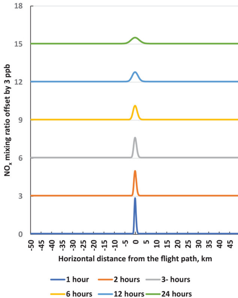
Figure 4.4: \text{NO}_x mixing ratios as a function of distance from the flight path at increasing times after the passage of an aircraft, each offset by 3 ppb.
