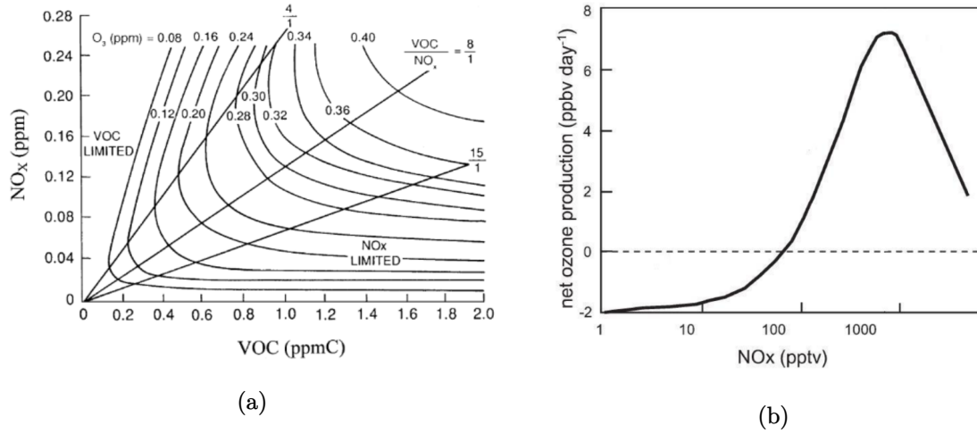
Figure 2.13: (a) Example isopleth diagram displaying peak ozone concentrations calculated from various initial concentrations of \text{NO}_x and a specified VOC mixture, using the US EPA empirical kinetic model [148, 149]. (b) Schematic representation of the variation of net ozone production efficiency with \text{NO}_x concentrations, with magnitudes reflecting clean free tropospheric conditions (i.e. low \text{VOC}/\text{NO}_x ratio) [146].
