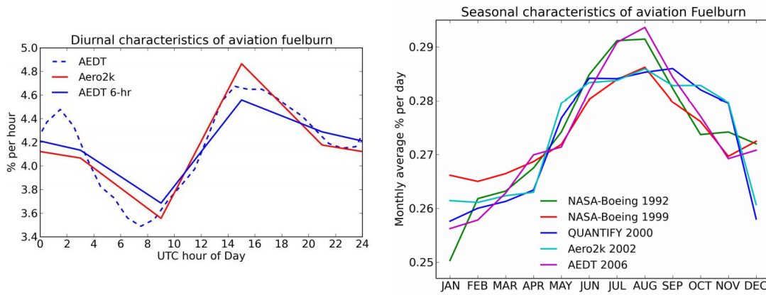
Figure 2.8: Temporal (diurnal and seasonal) distribution of global aviation fuel burn expressed as percentage from a range of aircraft emissions datasets [9].
