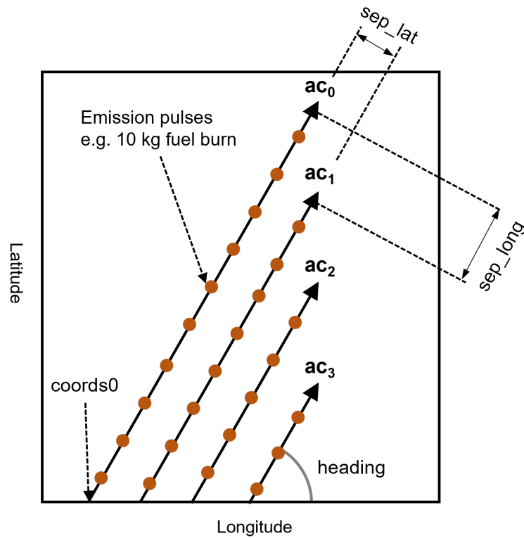
Figure 5.2: Schematic representation of GPAT flight trajectories for a four-aircraft formation configuration.
