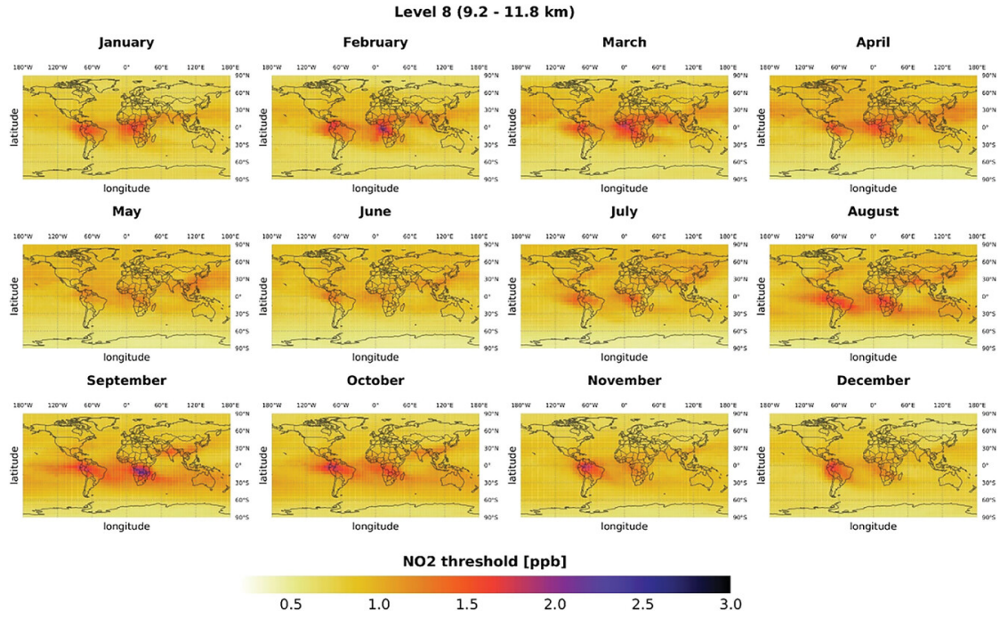
Figure 4.2: Global [\text{NO}_2]_{\text{equiv}} at model output level 8 (9.2–11.8 km) estimated using [\text{CH}_4] , [\text{CO}] , [\text{M}] , and temperature fields simulated by STOCHEM Common Representative Intermediate (CRI).
