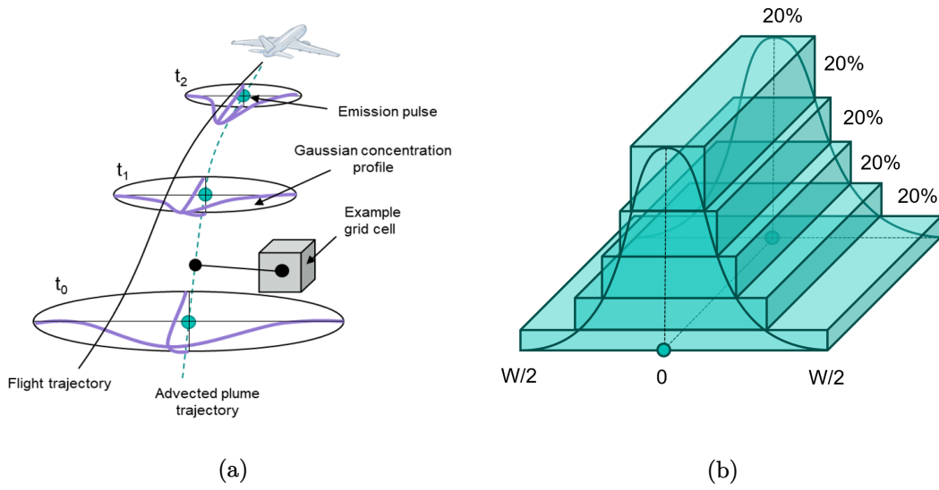
Figure 5.8: (a) Schematic representation of Gaussian dispersion and advection from GPAT plume simulations. (b) Five slice Gaussian aggregation to 2D Eulerian grid. Gaussian starts at half plume width ( W/2 ).
