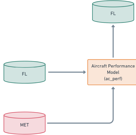
Figure 5.6: Process flow diagram for the Aircraft Performance Model. This takes in the first generation Flight Dataset and Meteorology Dataset, interpolated and down-selected to the trajectory waypoints. It outputs the second generation FL dataset, updated with performance characteristics.
