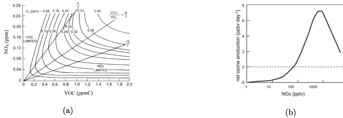
Figure 2.13: (a) Example isopleth diagram displaying peak ozone concentrations calculated from various initial concentrations of \text{NO}_x and a specified VOC mixture, using the US EPA empirical kinetic model [148, 149]. (b) Schematic representation of the variation of net ozone production efficiency with \text{NO}_x concentrations, with magnitudes reflecting clean free tropospheric conditions (i.e. low \text{VOC}/\text{NO}_x ratio) [146].
