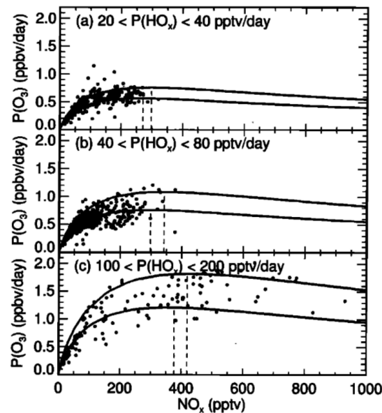
Figure 2.17: Empirical observations of ozone production rate as a function of NO_x concentrations (parts per trillion volume, pptv), for three ranges of primary HO_x production: (a) 20–40 pptv/day, (b) 40–80 pptv/day, and (c) 100–200 pptv/day. Solid lines represent the range limits from model calculations. Dashed lines depict the NO_x level that induces peak ozone response [19].
