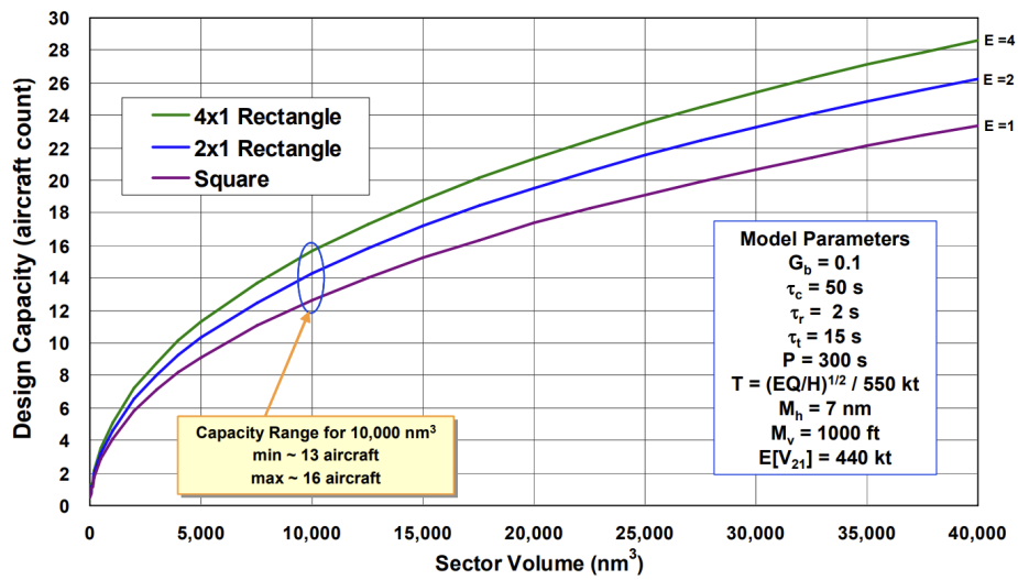
Figure 2.6: Aircraft capacity estimation against sector volume for a range of airspace scenarios [81]. E refers to the length-to-width ratio of the sector, G_b , \tau_c , \tau_r and \tau_t are all empirical parameters related to controller workload, P is the mean task recurrence period per aircraft, T is the sector transit time, M_h and M_v are the designated horizontal and vertical separation minima between aircraft within the sector and E[V_{21}] is the typical aircraft closing speed [82].
