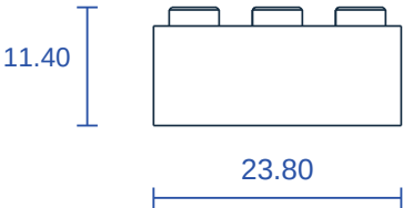
TOP / PRINT ORIENTATION
