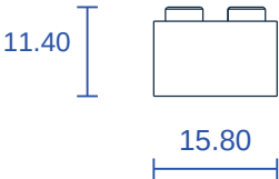
TOP / PRINT ORIENTATION
