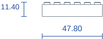
TOP / PRINT ORIENTATION
