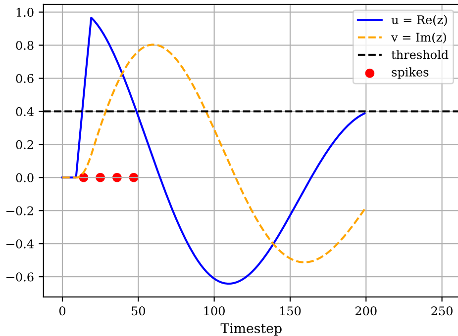
Classic Resonate-and-Fire
