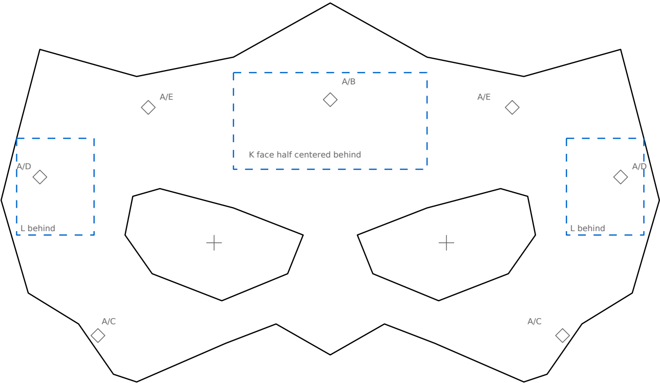
A x1 | 4 mm
