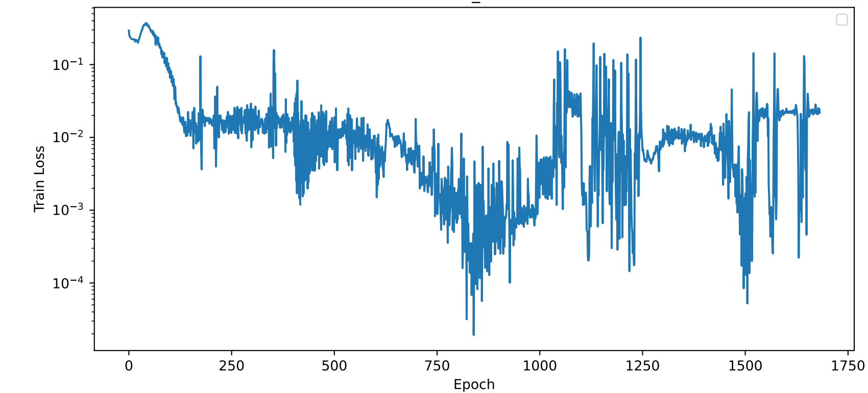
Train_Loss
