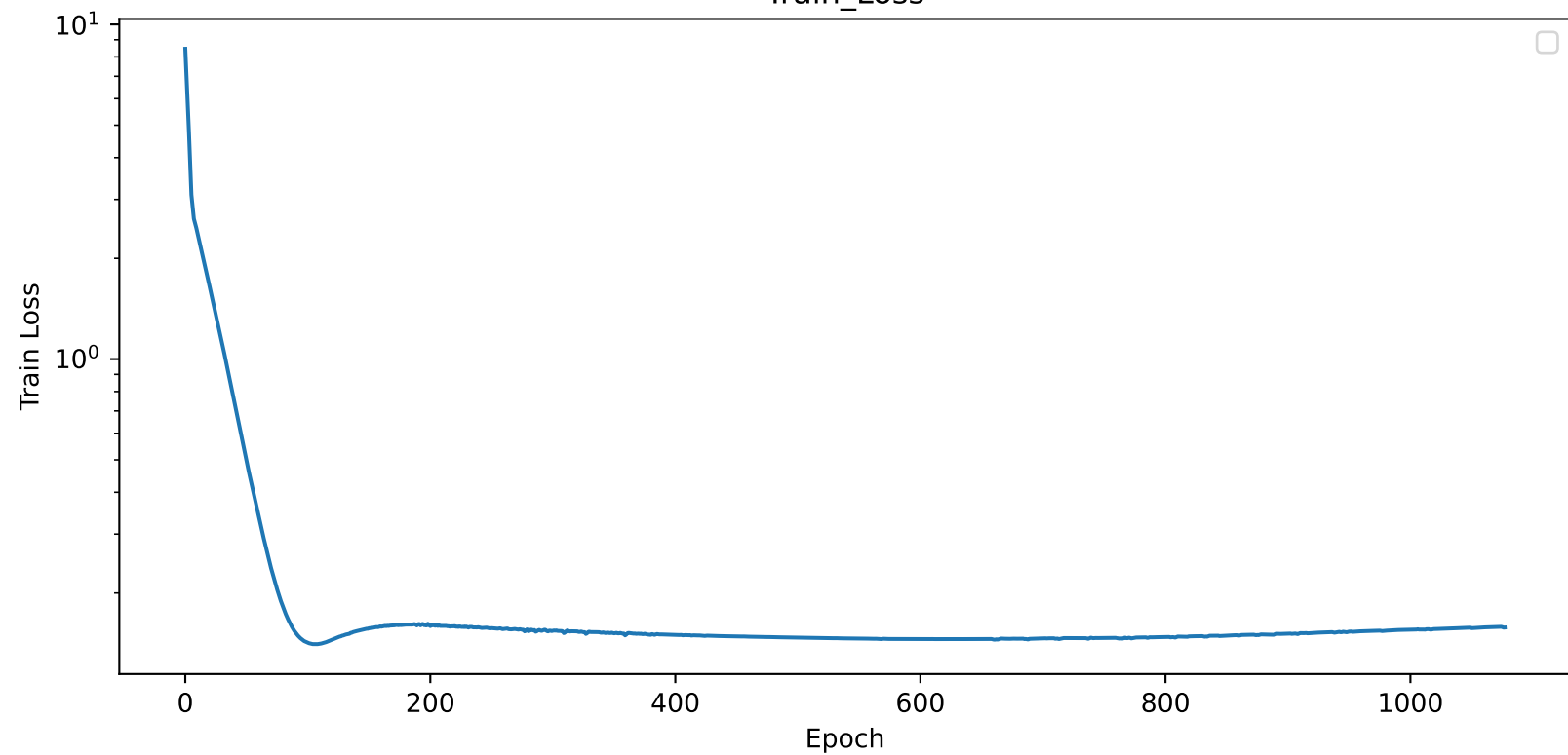
Train_Loss
