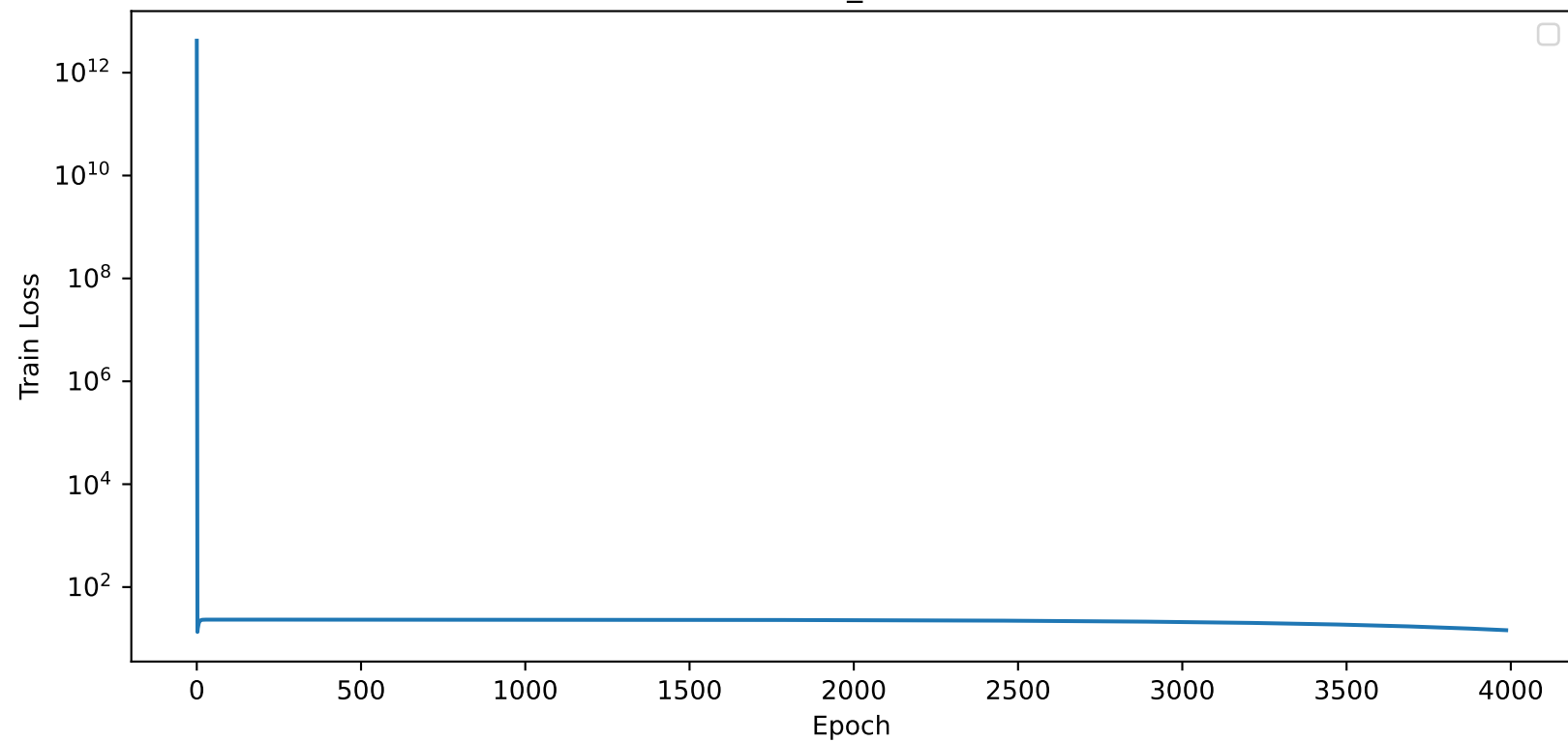
Train_Loss
