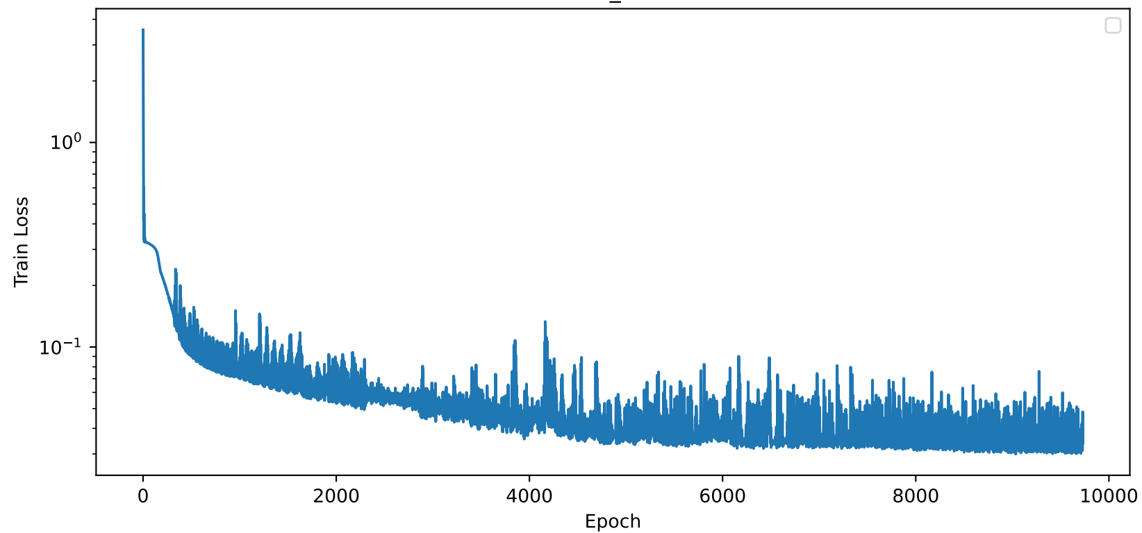
Train_Loss
