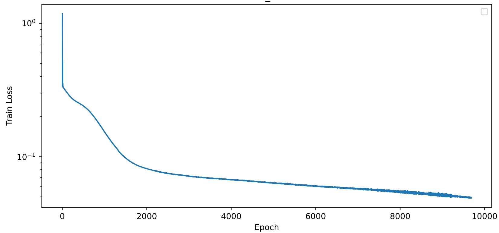
Train_Loss
