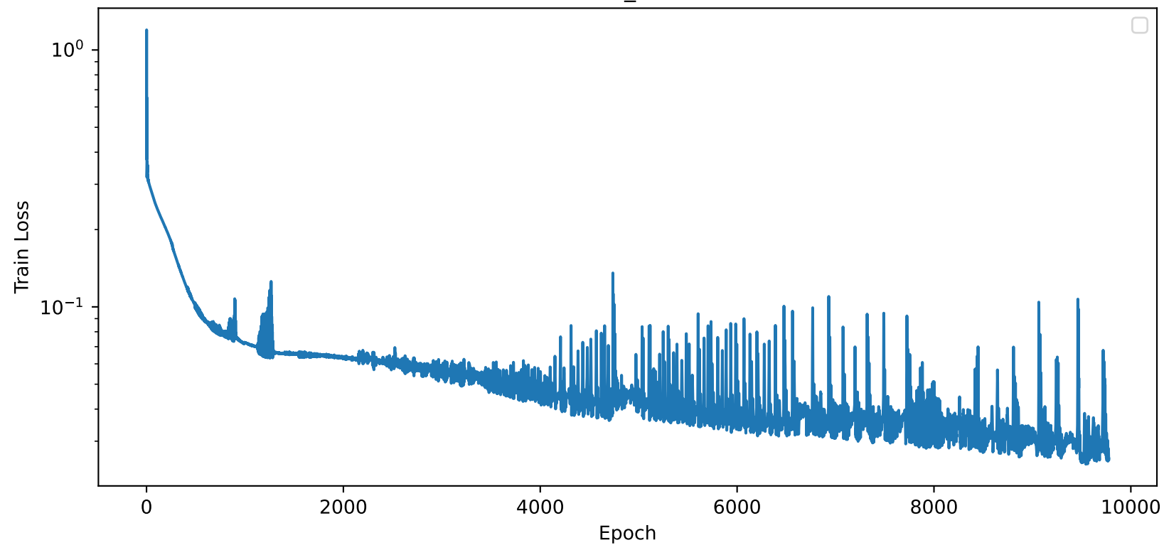
Train_Loss
