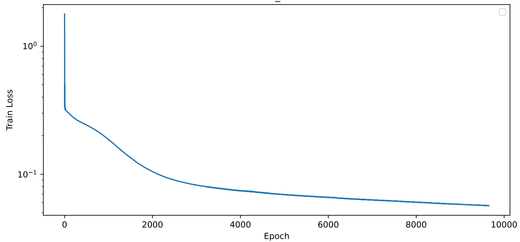
Train_Loss
