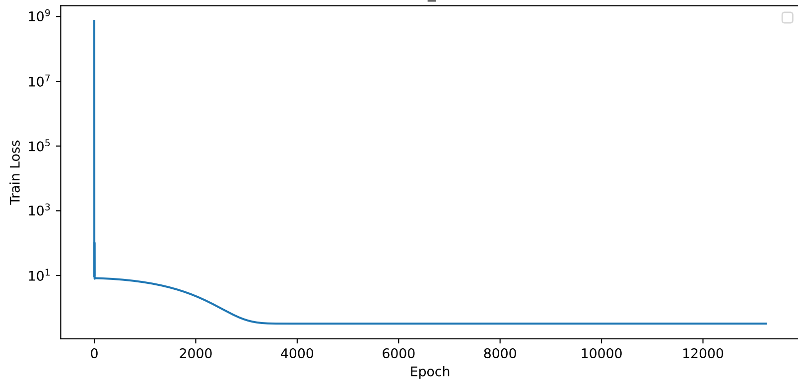
Train_Loss
