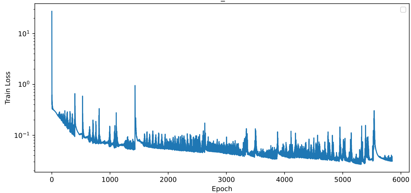
Train_Loss
