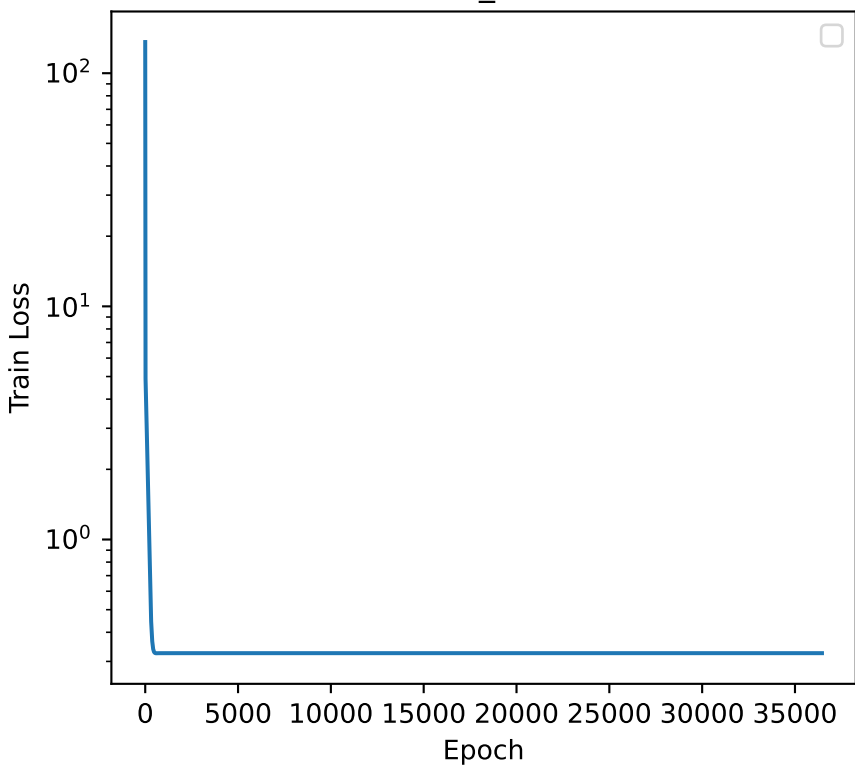
Train_Loss
