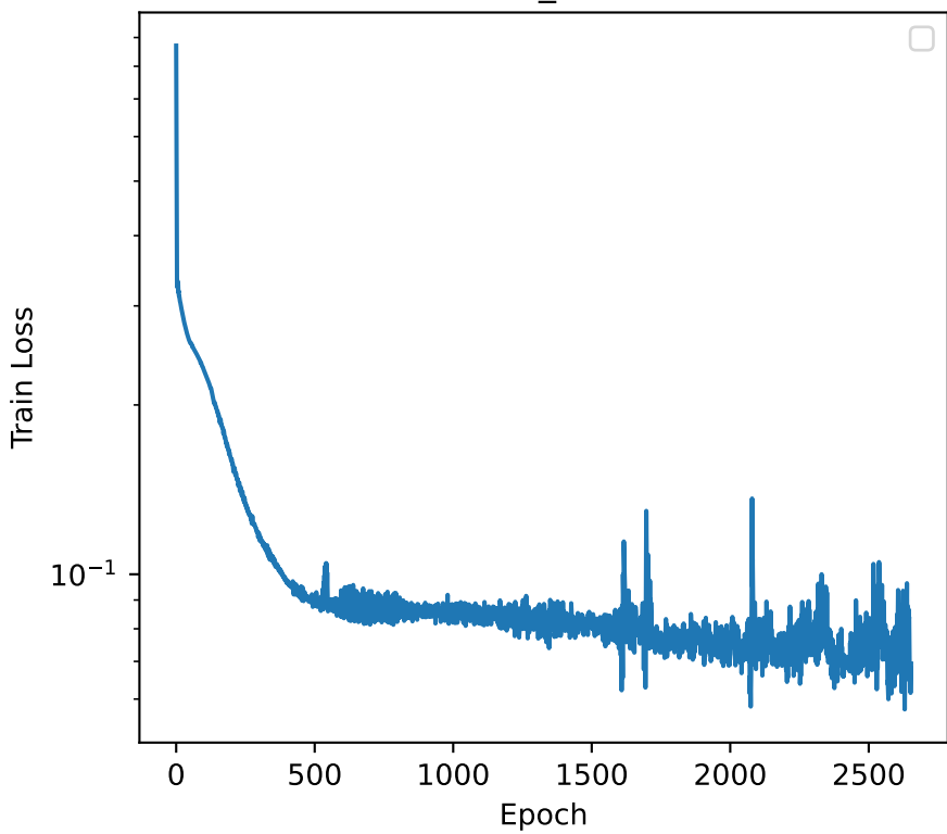
Train_Loss
