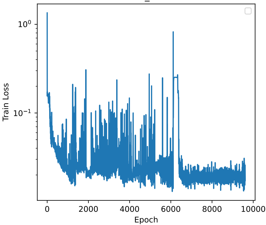
Train_Loss
