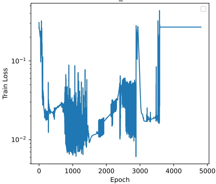
Train_Loss
