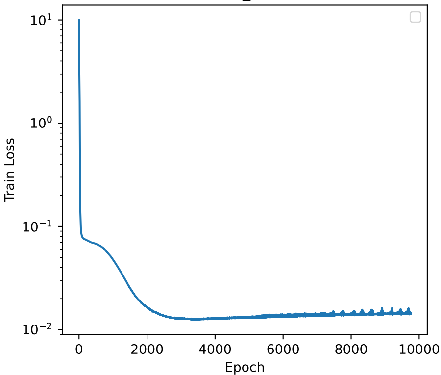
Train_Loss
