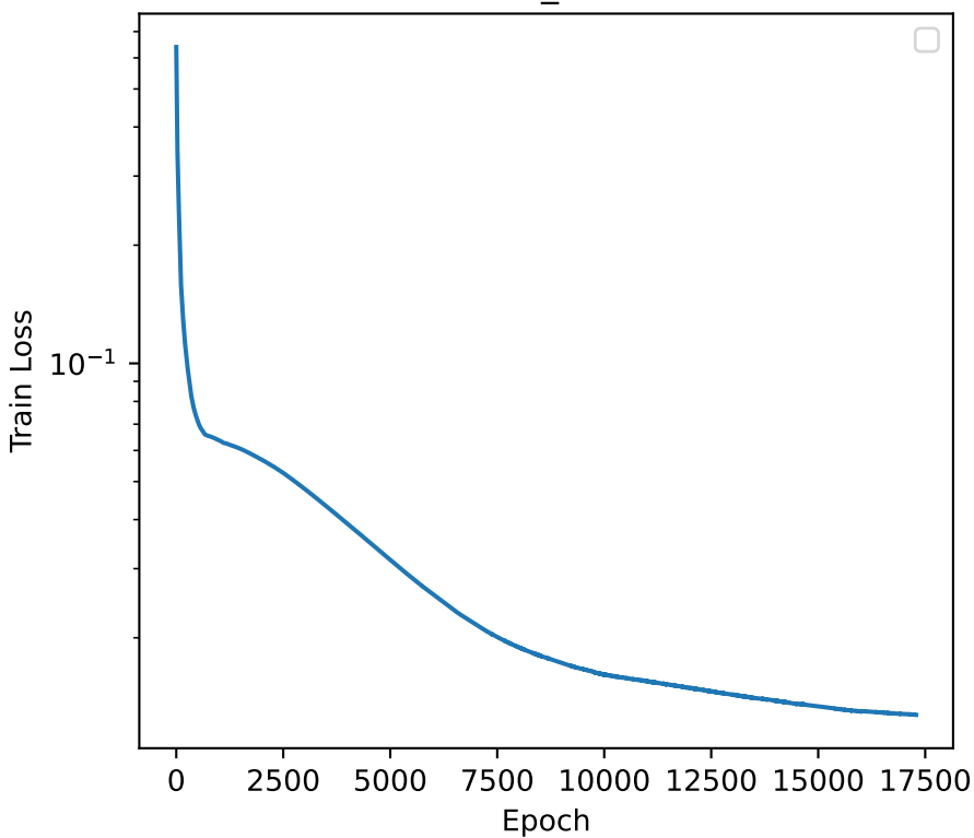
Train_Loss
