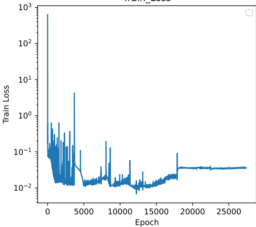
Train_Loss
