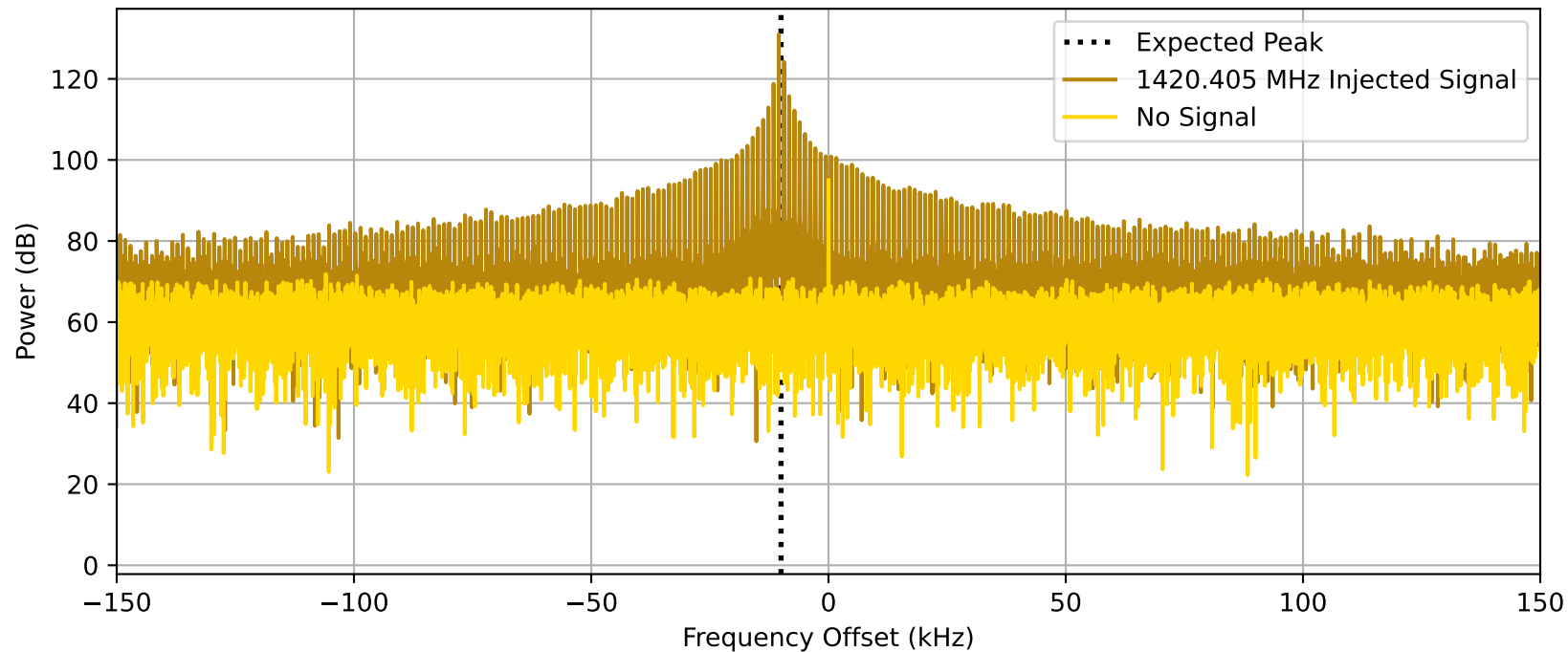
Baseband Power Spectrum with 1420 MHz Injected Signal (I/Q Data, Hann Window)
