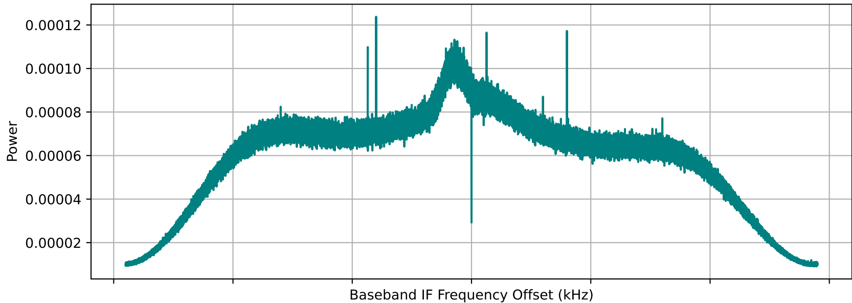
Averaged Baseband Power Spectrum (Blocks=1000)
