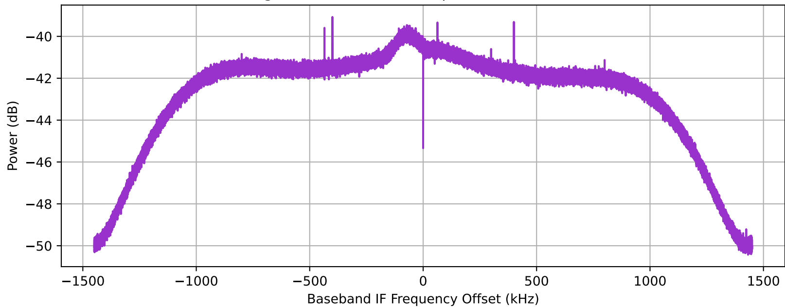
Averaged Baseband Power Spectrum (Blocks=1000)
