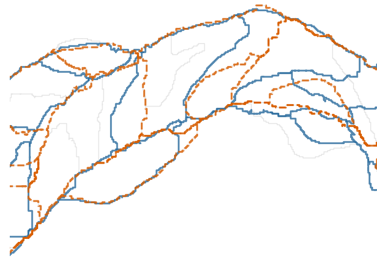
Hausdorff distance
