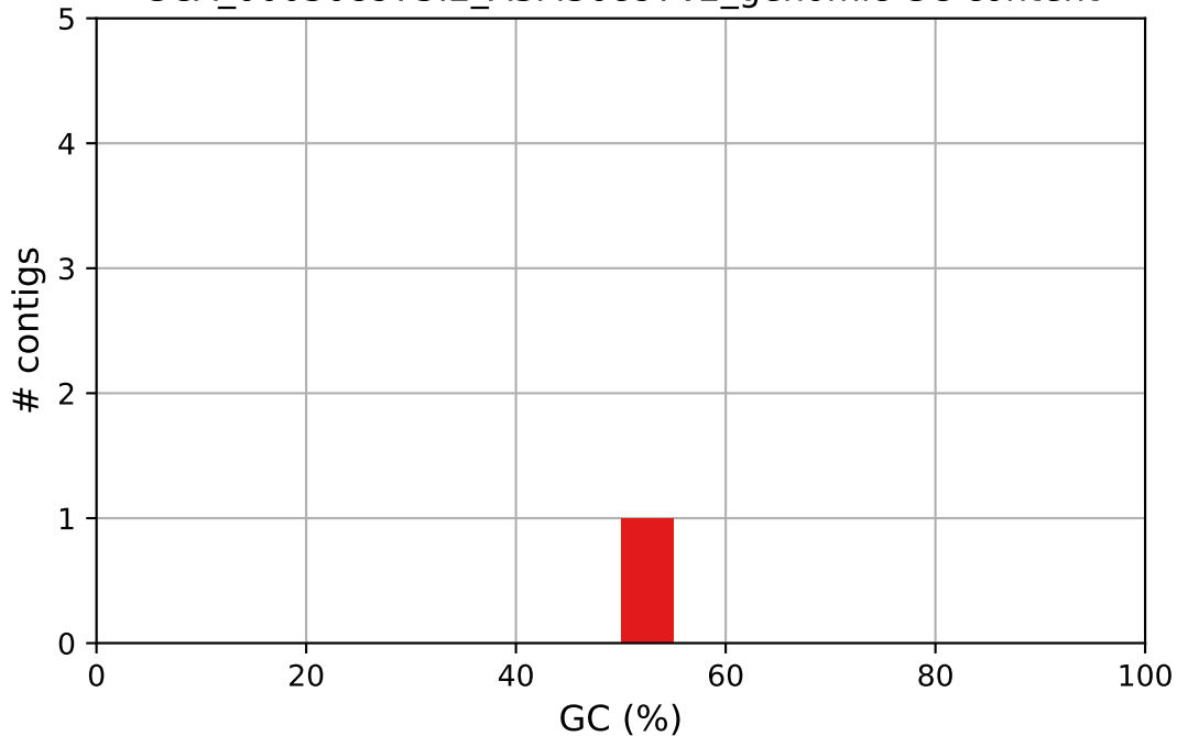
GCA_000308975.2_ASM30897v2_genomic GC content
