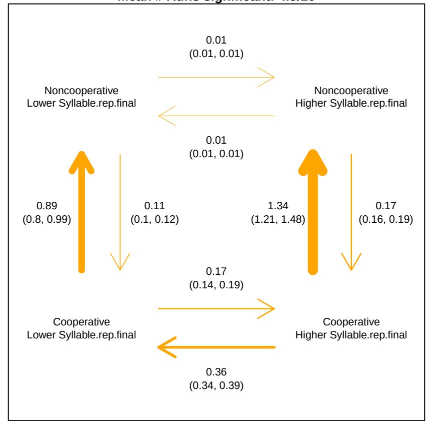
Thresholds \geq 12 - < 41.3 (29) Mean # Runs significant: 4.5/10
