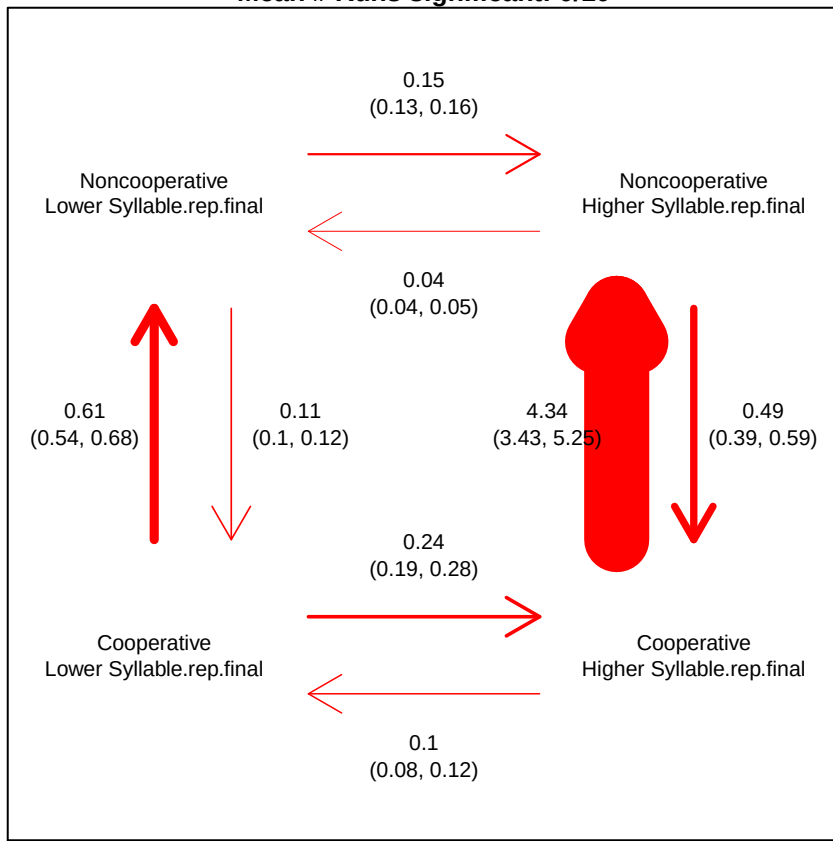
Thresholds \geq 1 - < 12 (28) Mean # Runs significant: 0/10
