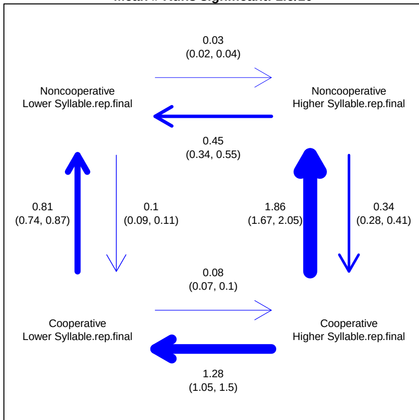
Thresholds \geq 41.3 - < 2400 (28) Mean # Runs significant: 1.6/10
