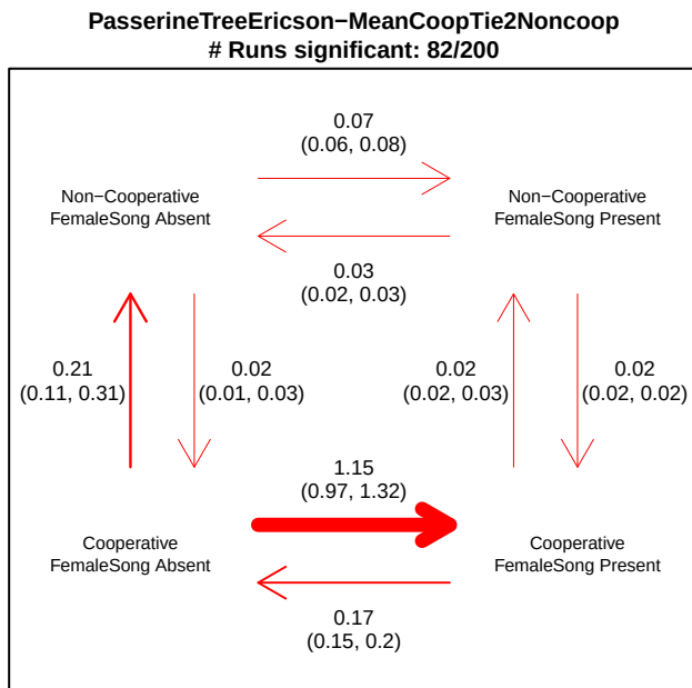
Gerygone_magnirostris CoopBreed was 1 now 0
