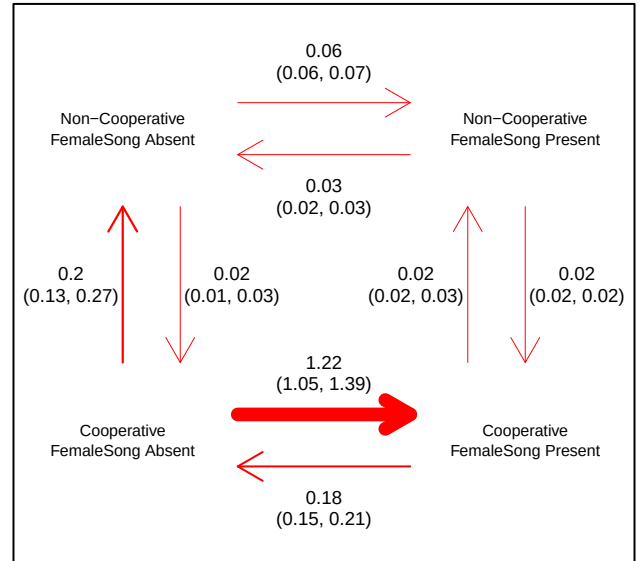
PasserineTreeEricson-MeanCoopTie2Noncoop # Runs significant: 89/200
