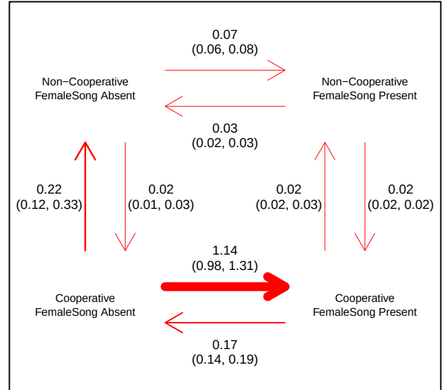
PasserineTreeEricson-MeanCoopTie2Noncoop # Runs significant: 81/200
