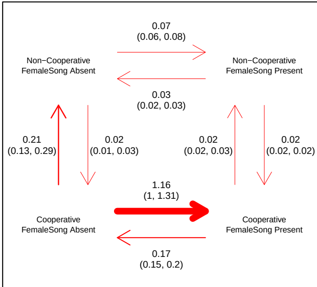
PasserineTreeEricson-MeanCoopTie2Noncoop # Runs significant: 90/200
