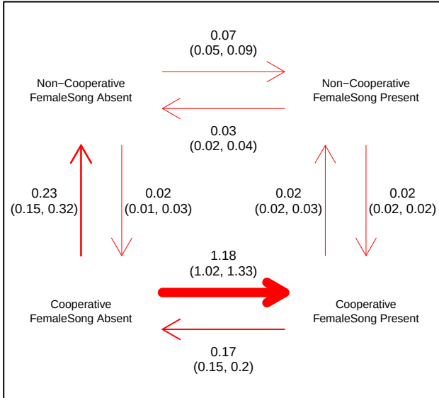
PasserineTreeEricson-MeanCoopTie2Noncoop # Runs significant: 73/200
