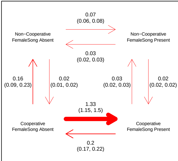
PasserineTreeEricson-MeanCoopTie2Noncoop # Runs significant: 86/200
