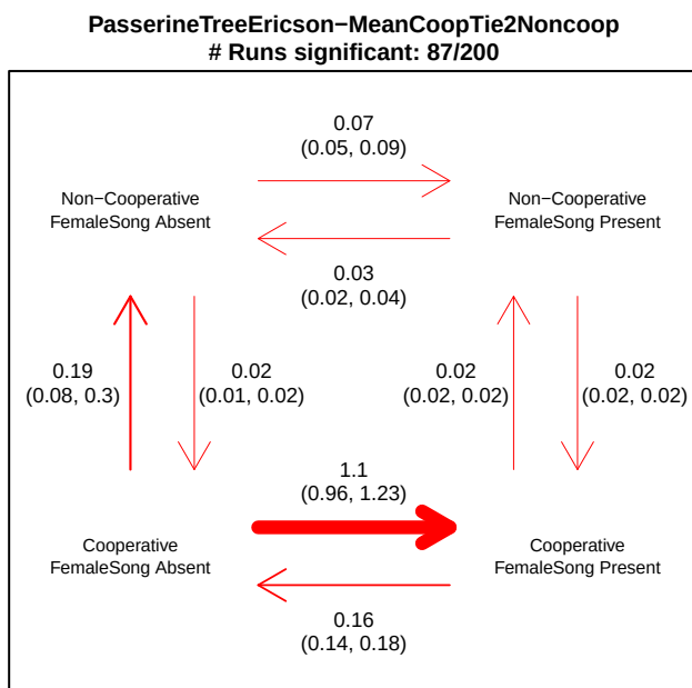
Lanius_collurio CoopBreed was 1 now 0
