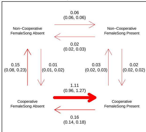
PasserineTreeEricson-MeanCoopTie2Noncoop # Runs significant: 71/200
