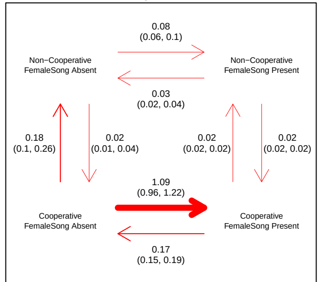
PasserineTreeEricson-MeanCoopTie2Noncoop # Runs significant: 83/200
