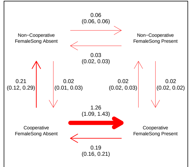
PasserineTreeEricson-MeanCoopTie2Noncoop # Runs significant: 82/200
