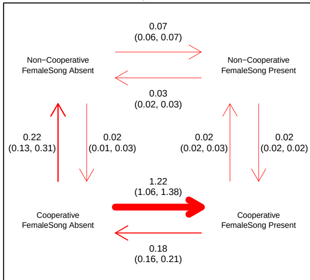
PasserineTreeEricson-MeanCoopTie2Noncoop # Runs significant: 83/200
