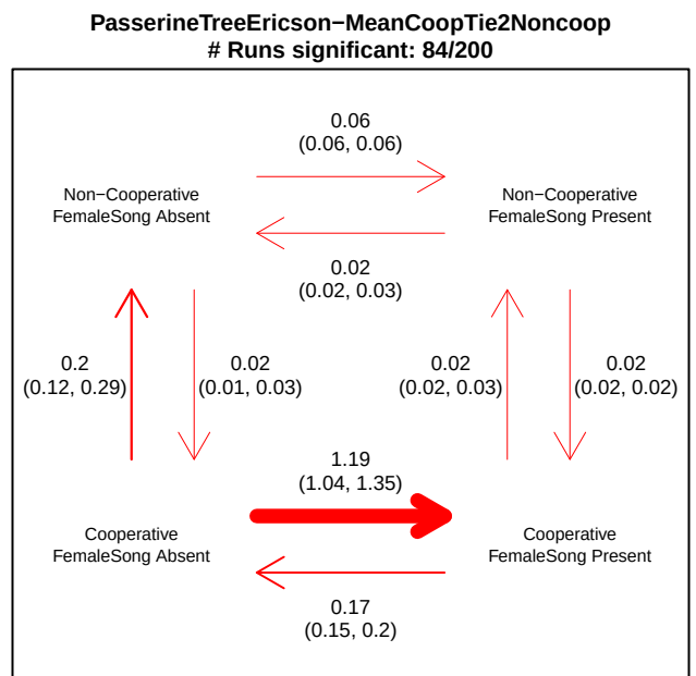
Conopophila rufogularis CoopBreed was 1 now 0
