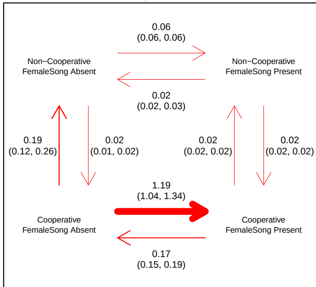
PasserineTreeEricson-MeanCoopTie2Noncoop # Runs significant: 78/200
