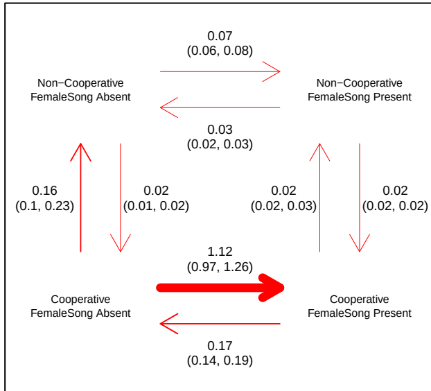
PasserineTreeEricson-MeanCoopTie2Noncoop # Runs significant: 80/200
