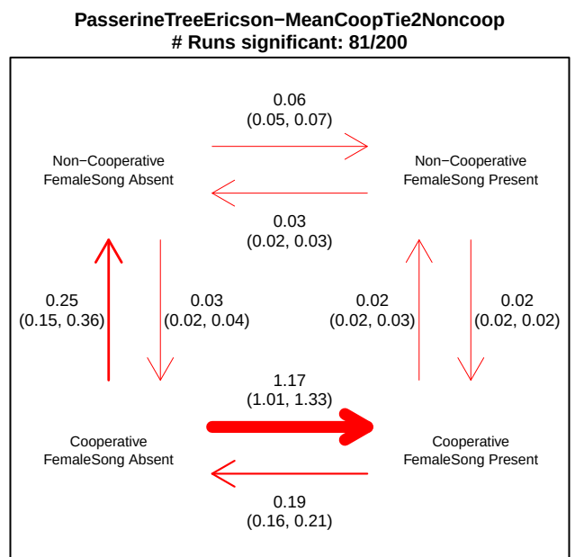
Lichenostomus flavescens CoopBreed was 1 now 0
