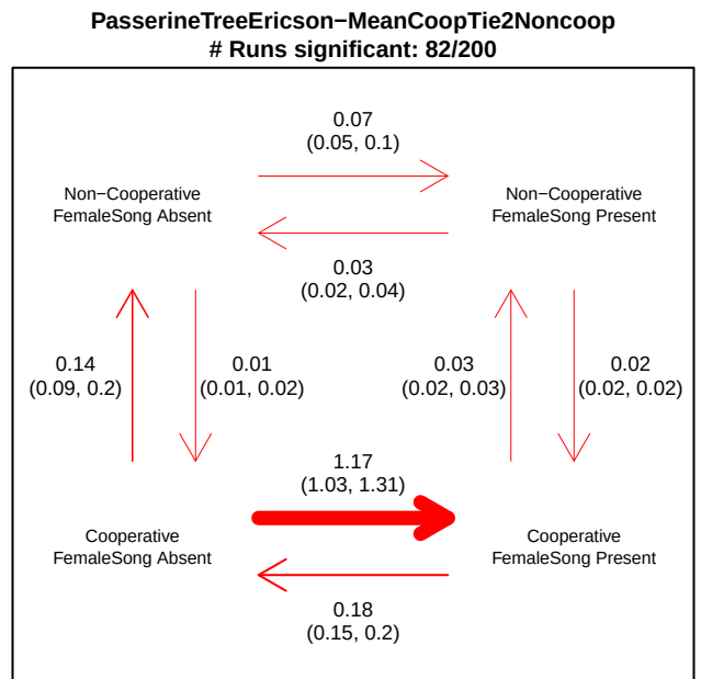
Lanius collaris CoopBreed was 1 now 0
