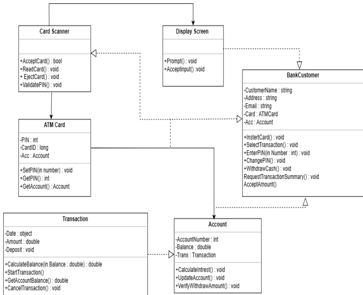
Class Diagram of ATM System
