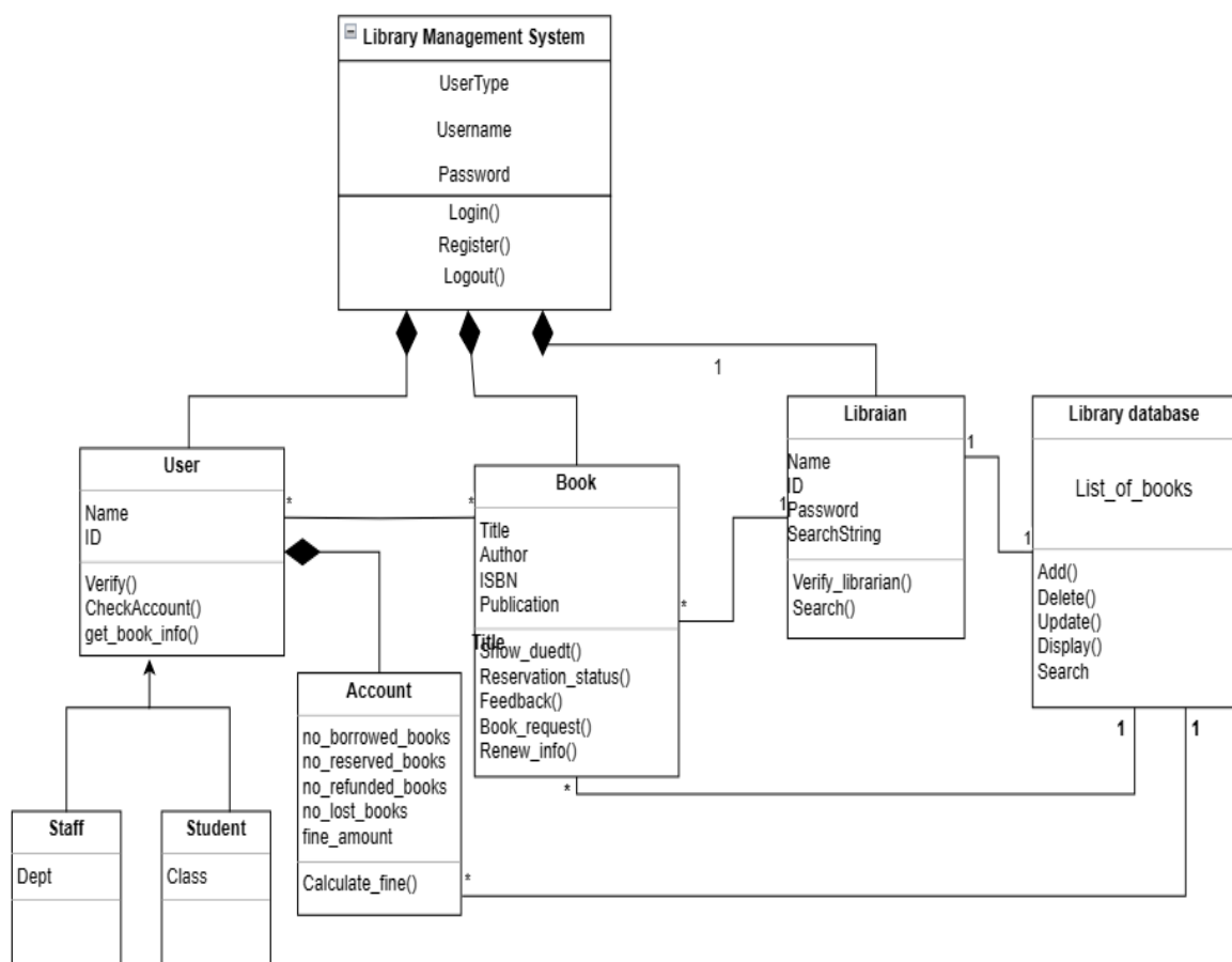
Class Diagram For Library Management System
